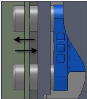
TWO SOLID STEEL BOLTS LOCKING SYSTEM
